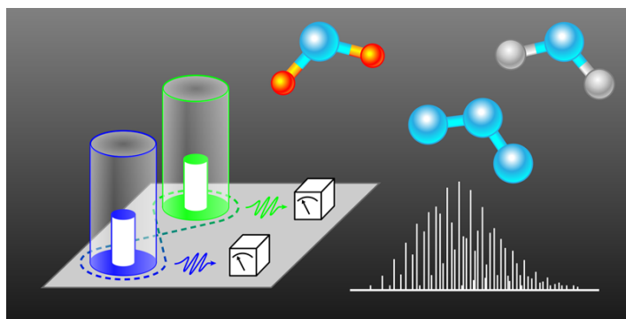
Figure 1: (Left) Sketch of the quantum simulator scheme used by Wang et al. [3], which is based on microwave photons confined to two resonant cavities (shown in blue and green). Photons in one cavity can be entangled with photons in the other cavity, and the photons’ quantum states can be detected nondestructively by two qubits (shown in orange) coupled to the cavities. (Right) The scheme generates the vibronic spectra of several triatomic molecules. (APS/Alan Stonebraker)
