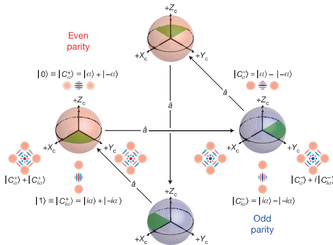
Figure 1 | The cat-code cycle. In the logical encoding of |0\rangle \equiv |C_\alpha^\pm\rangle = |\alpha\rangle \pm |-\alpha\rangle and |1\rangle \equiv |C_{i\alpha}^\pm\rangle = |i\alpha\rangle \pm |-i\alpha\rangle (normalizations omitted), the two ‘2-cats’ |C_\alpha^\pm\rangle and |C_{i\alpha}^\pm\rangle are eigenstates of either even (+) or odd (–) photon-number parity (an ‘n-cat’ is a superposition of n coherent states). For large enough |\alpha| they are effectively orthogonal to one another. In this basis, the states along the logical axes +X_c and +Y_c are both ‘4-cats’ of even or odd parity as well. The different patterns in the fringes of their cartoon Wigner functions signify the different phase relationship between the basis states. These features allow one to store a qubit in a superposition of 2-cats, |\psi\rangle = c_0|C_\alpha^\pm\rangle + c_1|C_{i\alpha}^\pm\rangle , and at the same time monitor the parity as the error syndrome without learning anything about c_0 or c_1 , the arbitrary coefficients satisfying |c_0|^2 + |c_1|^2 = 1 . In this example, we choose to encode |0\rangle and |1\rangle in the even-parity basis, although the odd basis can equally be chosen. The loss of a single photon changes not just the parity of the basis states (red shading, even; blue shading, odd), but the phase relationship between them by a factor of i as well: \hat{a}(c_0|C_\alpha^\pm\rangle + c_1|C_{i\alpha}^\pm\rangle) = c_0|C_\alpha^\pm\rangle + i c_1|C_{i\alpha}^\pm\rangle . Therefore, after one photon jump, one finds the initial qubit rotated by \pi/2 about the logical Z_c axis. With each subsequent application of \hat{a} , the encoded state cycles between the even- and odd-parity subspaces, while, owing to each consequent multiplication of the coefficient c_1 by i , the encoded information rotates about the Z_c axis by \pi/2 , as indicated by the rotation of the green shaded slice. Between the stochastic applications of \hat{a} , the cat states deterministically decay towards vacuum: \alpha \rightarrow \alpha e^{-\kappa t/2} (not depicted here), indicating that the logical basis changes in time.
