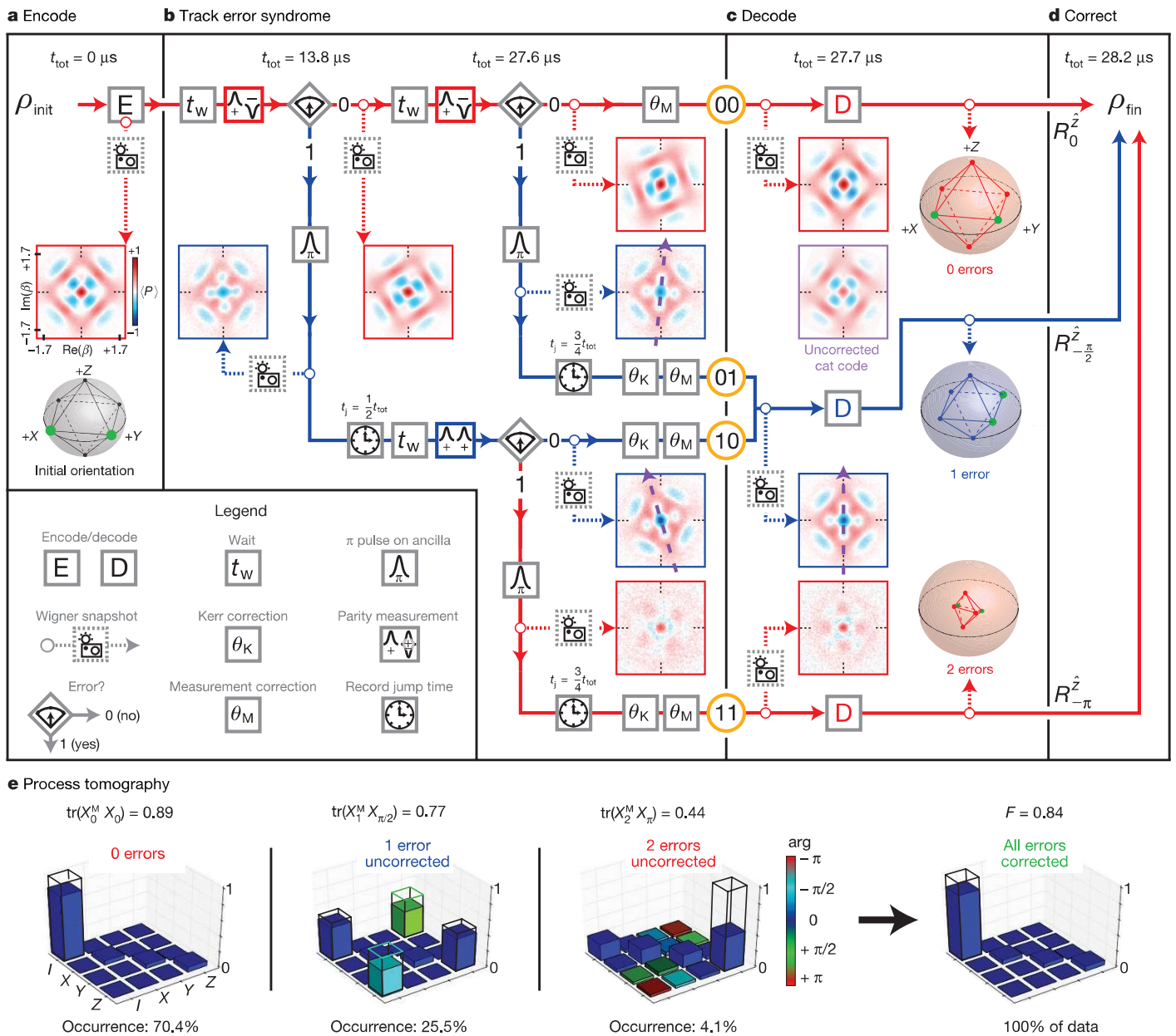
Figure 2 | Example of a two-step quantum trajectory executed by the QEC state machine. a , Six cardinal points on the Bloch sphere \rho_{\text{init}} are encoded ('E') from the ancilla onto even-parity resonator states; green markers indicate the initial coordinate-system orientation. A 'Wigner [tomography] snapshot' is shown for \frac{1}{\sqrt{2}}(|0\rangle - |1\rangle) \rightarrow \frac{1}{\sqrt{2}}(|C_{\alpha}^+\rangle - |C_{\alpha}^-\rangle) ; \bar{n}_0=3 ; \beta is the amplitude of varying coherent displacements ( \hat{D}_{\beta}|0\rangle_r = |\beta\rangle ) and the average parity \langle P \rangle = \langle \hat{D}_{\beta}^{\dagger} \hat{P} \hat{D}_{\beta} \rangle , where \hat{P} = e^{i\pi a^{\dagger} a} . b , A state machine for adaptive parity monitoring with delays t_w \approx 13 \mu\text{s} between each measurement. 'Parity measurement' rectangles show the Ramsey sequence that maps even [ +/- ] (odd [ +/+ ]) parity onto ancilla |g\rangle ( |e\rangle ); the + or - specifies the sign of the \pi/2 pulse. Diamonds indicate branching on ancilla measurement ( 0 \rightarrow no error, |g\rangle ; 1 \rightarrow error, |e\rangle ); ' \pi pulse on ancilla' rectangle indicates ancilla reset ( |e\rangle \rightarrow |g\rangle ); clocks indicate recording of the error time t_j . Dashed purple arrows emphasize the phase difference between 10 and 01 due to \theta_K . Rotations \theta_M are due to cross-Kerr interactions between the readout and storage resonators during ancilla
