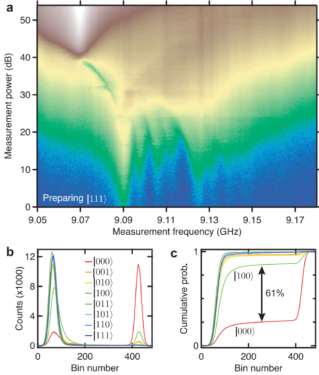
FIG. 3 (color). Joint qubit readout. (a) Pulsed cavity response \bar{A}_H when preparing the |111\rangle state. The eight ( 2^3 ) register states of three qubits induce a different dispersive cavity shift, each discernible at low power due to decay of the |111\rangle state during measurement. These frequencies were independently measured to be (f_{|000\rangle}, f_{|100\rangle}, f_{|010\rangle}, f_{|001\rangle}, f_{|110\rangle}, f_{|101\rangle}, f_{|011\rangle}, f_{|111\rangle}) = (9.145, 9.139, 9.131, 9.112, 9.124, 9.105, 9.097, 9.090) GHz, with f_{\text{bare}} = 9.070 GHz. The most prominent secondary cavity position corresponds to the third qubit (at 8 GHz) relaxing during measurement, consistent with its Purcell-limited [32] T_1 being shortest of the three, with T_1^{Q_1} = 1.2 \mu\text{s} , T_1^{Q_2} = 1.0 \mu\text{s} , and T_1^{Q_3} = 0.6 \mu\text{s} . The system excites to its bright state at lower power here than seen in Fig. 1 because of the smaller initial cavity detuning from f_{\text{bare}} . The color scale is identical to that in Fig. 1. (b) Histograms for all eight basis states, when driving with +49 dB at f_{\text{bare}} . (c) S curves for joint qubit readout, indicating a minimum of 61% fidelity for distinguishing the |000\rangle from any other state. The best fidelity in this case is obtained with a \sim 25\% probability of exciting the system when prepared in |000\rangle .
