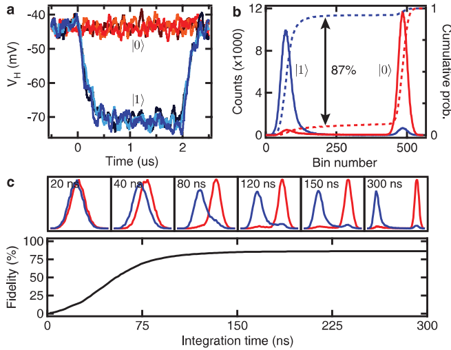
FIG. 2 (color). Measurement transients and histograms for single-shot measurement of one qubit (at 8 GHz). (a) Three measurements of single-shot system response V_H(t) to driving at f_{\text{bare}} with a power P_{\text{meas}} for prepared qubit ground and excited states, low-passed to the response time of the cavity 1/\kappa \approx 100 ns. They are reproducible and well distinguished, demonstrating that the response is large compared to the measurement noise. (b) Histograms and S curves quantifying measurement fidelity. An ensemble of single-shot responses are integrated for 500 ns and their distribution plotted. The two histogram peaks (solid lines) are well separated with few counts between them. Integrating these yields “ S curves” (dashed lines), with their maximal difference indicating a single-shot fidelity of 87%. (c) Measurement fidelity versus integration time. Integrating V_H(t) for 120 ns yields 80% fidelity, while 240 ns yields 87%. The histogram evolution shows that integrating longer further separates the peaks but does not increase fidelity.
