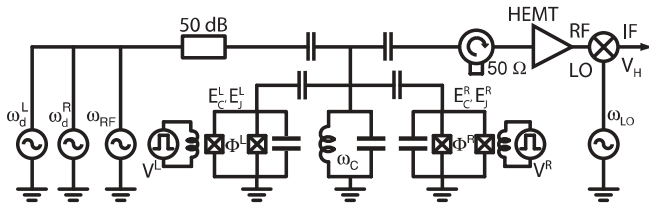
FIG. 5. Circuit diagram of experimental setup, showing the cavity as a lumped LC resonator. Microwave drive tones that address the cavity, \omega_{\text{RF}} , and qubits, \omega_{\text{d}}^{L(R)} , are applied via the cavity input line. The left (right) qubit, with Josephson energy E_J^{L(R)} and charging energy E_C^{L(R)} , is tunable via a local flux \Phi^{L(R)} set by a voltage V^{L(R)} . The joint qubit state information is transmitted out a single readout line, amplified through a high electron mobility transistor (HEMT) amplifier at 4 K and mixed down at room temperature for digital processing.
