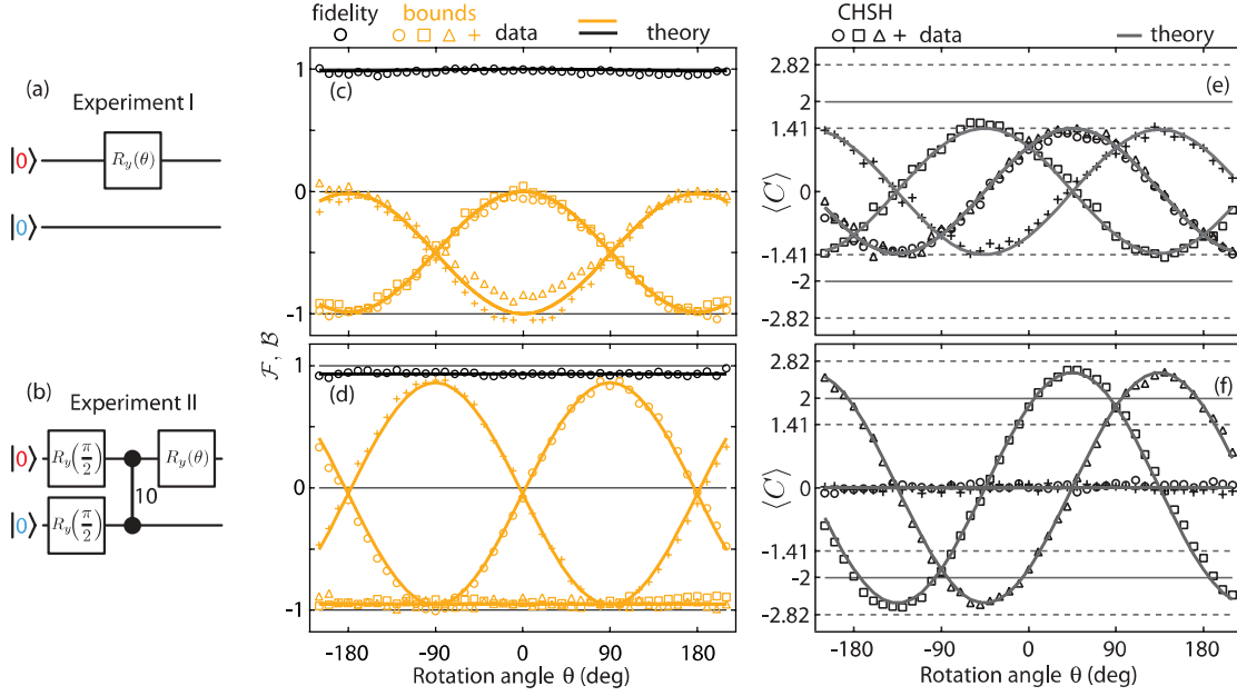
FIG. 4. (Color online) Pulse sequences for a collection of (a) separable and (b) entangled states, showing experimental lower bounds \mathcal{B}_i (orange) on concurrence given by the optimal witnesses for Bell states \mathcal{W}_{\psi_+} (circles), \mathcal{W}_{\psi_-} (squares), \mathcal{W}_{\phi_+} (triangles), and \mathcal{W}_{\phi_-} (crosses), and fidelity \mathcal{F} to the ideal state (black circles) for (c) experiment I and (d) experiment II. In (d), a maximum lower bound is reached by \mathcal{B}_{\psi_-} ( \mathcal{B}_{\psi_+} ) at \theta = -90^\circ ( +90^\circ ). Shown are four measured CHSH operators, \langle C_{ZZXX} \rangle (squares), \langle C_{XXZZ} \rangle (triangles), \langle C_{ZZXX} \rangle (circles), and \langle C_{XXZZ} \rangle (crosses), for a collection of (e) separable and (f) entangled states. Experiment I in (e) involves only a single qubit rotation and all \langle C \rangle values stay within the separable state bounds \pm\sqrt{2} up to measurement noise. For experiment II in (f), there are three single-qubit rotations and a c-Phase, and we find \max |\langle C \rangle| = 2.61 \pm 0.04 . Solid curves are the results of master equation simulations.
