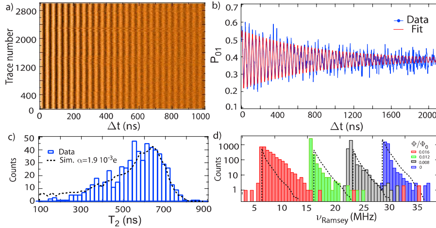
FIG. 5. (Color online) (a) 3000 Ramsey oscillations as a function of free evolution time \Delta t . Each trace is 2.1 \mu\text{s} long with 3 ns per step. They each take 0.35 s to acquire. We can see visually the variation of T_2 for the different Ramsey fringes by noticing the variation in contrast in the fringes near 1 \mu\text{s} . (b) Sample data fit. We average five of the acquired Ramsey traces shown in (a) and fit to a decaying sinusoid to extract the T_2 which is then plotted in (c). For this particular case, we have a coherence time of 840 ns and a Ramsey frequency of 26.9 MHz. (c) Distribution of T_2 for 3000 of the Ramsey traces (600 fits). The black dashed line is the result of a simulation of the free evolution decay of the Ramsey fringes with 1/f noise fluctuations on the gate, S_q(\omega) = \alpha^2/|\omega| . In the simulation, we used ten times more points compared to the data to obtain a smoother curve. (d) Corresponding distribution of Ramsey frequencies at four different flux biasing points. Each distribution has 3000 Ramsey traces. The blue histogram corresponds to the data in (a), (b), and (c). The Ramsey frequency is extracted from the position of the maximum of the power spectral density of each decaying sinusoid. The distributions are lopsided to higher frequencies as would be expected from fluctuations in the gate charge around our operating point at the sweet spot. The dashed line is the expected distribution assuming the same 1/f charge noise as in (c).
