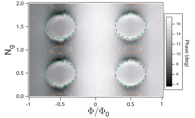
FIG. 2. (Color online) Gate charge and flux modulations of our device. We operated in the weakly nonlinear mode ( P \ll P_b^{(1)} ) and monitored the phase of the transmitted signal (grayscale) as we varied the applied gate charge N_g = C_g V_g / 2e and flux \Phi ( \Phi_0 = \hbar/2e ). The large ellipsoidal contours can be interpreted as induced transitions between the energy levels of the qubit at multiples of the readout frequency. The green fitted lines are transitions between the 0 and 1 energy levels at the readout frequency of 9.64 GHz, while the orange fits are for transitions between the 0 and 2 energy levels at twice the readout frequency, 19.28 GHz.
