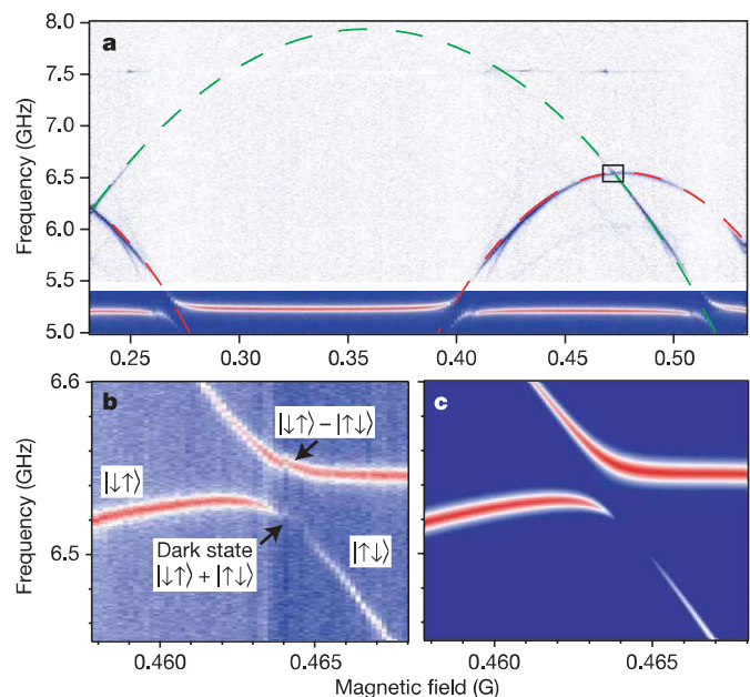
Figure 2 | Cavity transmission and spectroscopy of single and coupled qubits. a, The transmission through the cavity as a function of applied magnetic field is shown in the frequency range between 5 and 5.4 GHz. When either of the qubits is in resonance with the cavity, the cavity transmission shows an avoided crossing due to the vacuum Rabi splitting. The maximal vacuum Rabi splitting for the two qubits is the same within the measurement uncertainty and is \sim 105 MHz. Above 5.5 GHz, spectroscopic measurements of the two qubit transitions are displayed. A second microwave signal is used to excite the qubit and the dispersive shift of the cavity frequency is measured. The dashed lines show the resonance frequencies of the two qubits, which are a function of the applied flux according to \omega_{1,2} = \omega_{1,2}^{\max} \sqrt{|\cos(\pi\Phi/\Phi_0)|} . The maximum transition frequency for the first qubit is \omega_1^{\max}/2\pi = 7.8 GHz and for the second qubit is \omega_2^{\max}/2\pi = 6.45 GHz. For strong drive powers, additional resonances between higher qubit levels are visible. The black box indicates the region shown in b. b, Spectroscopy of the two-qubit crossing. The qubit levels show a clear avoided crossing with a minimum distance of 2J/2\pi = 26 MHz. At the crossing the eigenstates of the system are symmetric and antisymmetric superpositions of the two qubit states. The spectroscopic drive is antisymmetric and therefore unable to drive any transitions to the symmetric state, resulting in a dark state. c, Predicted spectroscopy at the qubit–qubit crossing using a markovian master equation that takes into account higher modes of the cavity. The parameters for this calculation are obtained from the vacuum Rabi splitting and the single-qubit spectroscopy.
