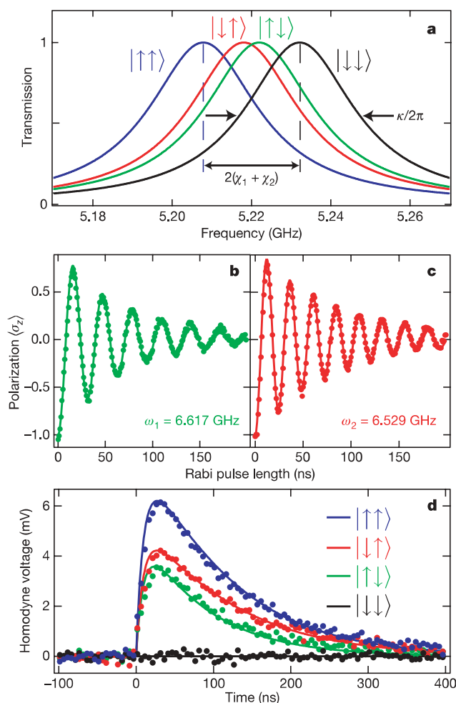
Figure 3 | Multiplexed control and read-out of uncoupled qubits. a , Predicted cavity transmission for the four uncoupled qubit states. In the dispersive limit ( |\Delta_{1,2}| = |\omega_{1,2} - \omega_r| \gg g_{1,2} ) the frequency is shifted by \chi_1\sigma_1^z + \chi_2\sigma_2^z . Operating the qubits at transition frequencies \omega_1/2\pi = 6.617 GHz and \omega_2/2\pi = 6.529 GHz, we find \chi_1/2\pi = -5.9 MHz and \chi_2/2\pi = -7.4 MHz. Measurement is achieved by placing a probe at a frequency where the four cavity transmissions are distinguishable. The two-qubit state can then be reconstructed from the homodyne measurement of the cavity. Rabi oscillations of qubit 1 ( b ) and qubit 2 ( c ) are shown. A drive pulse of increasing duration is applied at the qubit transition frequency and the response of the cavity transmission is measured after the pulse is turned off. Oscillations of quadrature voltages are measured for each of the qubits and mapped onto the polarization \langle\sigma_{1,2}^z\rangle . The solid line shows results from a master equation simulation, which takes into account the full dynamics of the two qubits and the cavity. The absence of beating in both traces is a signature of the suppression of the qubit–qubit coupling at this detuning. d , The homodyne response (average of 1,000,000 traces) of the cavity after a \pi -pulse on qubit 1 (green), qubit 2 (red), and both qubits (blue). The black trace shows the level when no pulses are applied. The contrasts 28 (that is, the amplitude of the pulse relative to its ideal maximum value) for these pulses are 60% (green), 61% (red) and 65% (blue). The solid line shows the simulated value, including the qubit relaxation and the turn-on time of the cavity. The agreement between the theoretical prediction and the data indicates that the measured contrast is the maximum observable. From the theoretical calculation we can estimate the selectivity (see text for details) for each \pi -pulse to be 87% (qubit 1) and 94% (qubit 2). We note that this figure of merit is not at all intrinsic and that it could be improved by increasing the detuning between the two qubits for instance, or using shaped excitation pulses.
