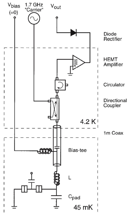
Fig. 3. The setup of the experiment.
