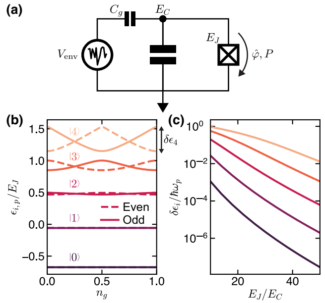
FIG. 1. Offset-charge dispersion of OCS-transmon eigenstates. (a) The circuit diagram of a Cooper-pair box or transmon coupled to charges in the environment. Fluctuating charges in the environment produce a noisy reduced-charge offset n_g = C_g V_{\text{env}}/2e , where C_g is an effective gate capacitance and e is the electron charge. The symbols E_J and E_C refer to the Josephson and charging energies, respectively, while \hat{\varphi} and P denote the difference in superconducting phase across the junction and the number parity of QPs that have tunneled across the junction, respectively. (b) The eigenenergies \epsilon_{i,p} of the Cooper-pair-box Hamiltonian with E_J/E_C = 17 , as a function of n_g , normalized by E_J . Solid (dashed) lines indicate the manifold of states corresponding to odd (even) charge parity. (c) The maximum charge dispersion \delta\epsilon_i of the five lowest energy levels, normalized by the plasma frequency \omega_p = \sqrt{8E_J E_C}/\hbar .
