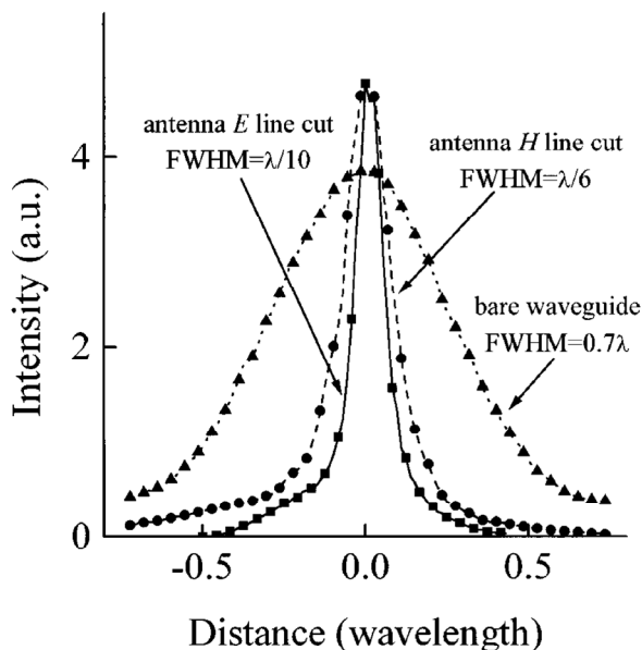
FIG. 3. Line cuts through the images in Fig. 2. The bare waveguide (triangles) shows a full width half-maximum (FWHM)= 0.7\lambda . The \mathbf{E} -direction line cut (squares) and the \mathbf{H} -direction line cut (circles) through the antenna image, Fig. 2(b), have a FWHM of \lambda/10 and \lambda/6 , respectively, clearly demonstrating that the antenna is acting as a near-field optical source.
