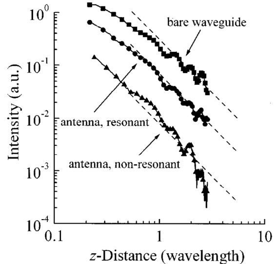
FIG. 4. Plots of the radiated power along the z -direction (i.e., axial) for the bare waveguide (squares), the antenna positioned resonantly with respect to the open end of the waveguide (circles), and the antenna positioned non-resonantly (triangles). The dashed lines are drawn as an aid to the reader and indicate inverse square law power dependence. The ratio of the nonresonant data to the bare waveguide data yields a transmission efficiency of order two percent, while the ratio of the resonant data to the bare waveguide data yields a transmission efficiency of order 30% .
