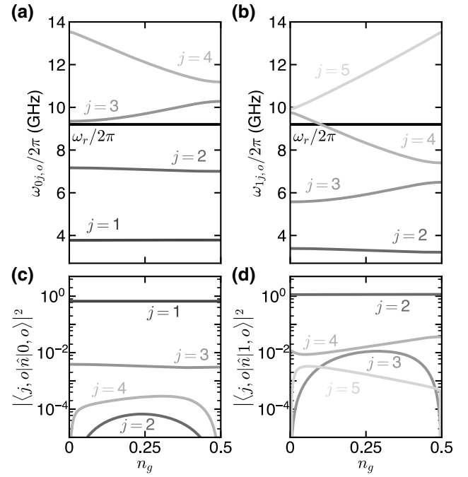
FIG. 2. The theoretically calculated OCS-transmon-readout spectrum as a function of n_g . (a),(b) The plasmon-transition frequencies out of the ground state (a) and the first excited state (b) of an OCS transmon with E_J/E_C = 17 with odd charge parity. In this parameter regime, the detuning between \omega_{03,o} and the resonator frequency \omega_r varies by a factor of approximately 8 as a function of the parameter n_g . Additionally, \omega_{14,o} crosses \omega_r near n_g = 0.1 . (c),(d) The matrix elements of the transmon charge operator for transitions out of the ground (c) and first excited state (d) with “odd” charge parity. These matrix elements are finite and relevant for calculating the transmon-readout dispersive shifts in our devices. In the transmon limit of large E_J/E_C , matrix elements between non-nearest-neighbor states will be suppressed.
