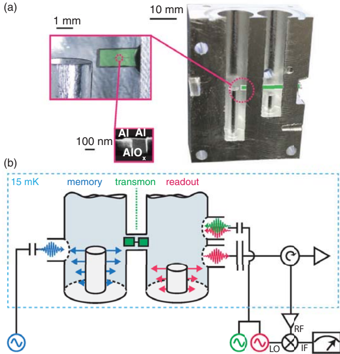
FIG. 2. Quantum memory and experiment scheme. To realize a quantum memory, a superconducting transmon qubit on sapphire (green) is inserted through small hole. (a) False-colored image showing a cross section of the system, with insets that show the transmon chip and a micrograph of the junction. (b) Schematic of the experiment. The transmon is coupled to the memory cavity as well as a second cavity used for readout. Weakly coupled pins are used for input signals (depicted as small capacitors). The measurement signal is extracted via a pin coupled strongly to the readout resonator (large capacitor) and amplified by a Josephson parametric converter (JPC) at base temperature of the dilution refrigerator, and subsequently demodulated using the readout oscillator (LO) as reference.
