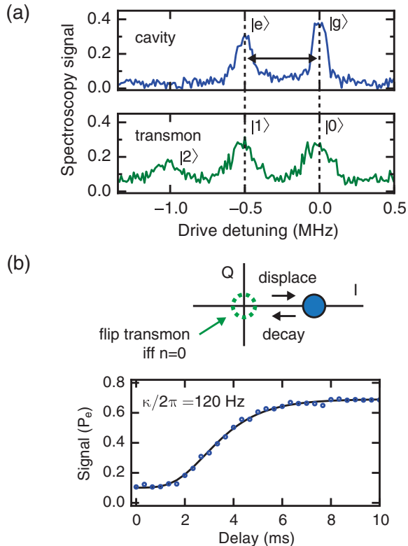
FIG. 3. Initial characterization of the cavity-transmon system. (a) With strong dispersive coupling, the spectrum of the resonator depends on the state of the transmon (top) and vice versa (bottom). (b) (top) The decay rate of the resonator can be measured by monitoring the population of the vacuum state after displacing the resonator; the state is schematically represented as a blue circle in the IQ plane of the resonator. (bottom) From the population decay we extract a decay rate of \kappa/2\pi = 120 \pm 5 Hz; see main text for details.
