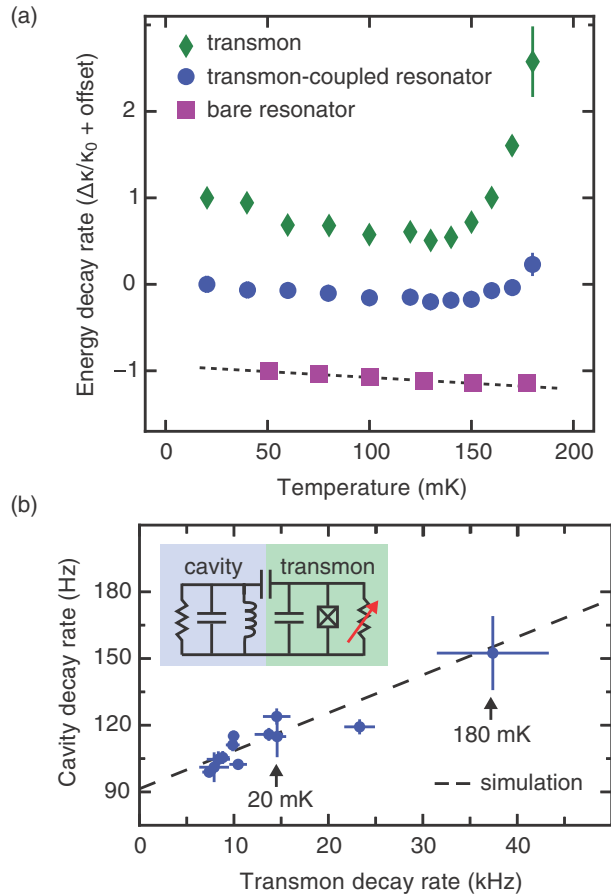
FIG. 6. Transmon-induced dissipation. The resonator inherited a photon-loss channel from coupling to the lossy transmon qubit. This effect can be revealed by tuning the decay rates in situ . (a) We monitor the decay rates of the transmon (green diamonds), transmon-coupled memory resonator (blue circles), and an empty resonator (purple squares) as a function of temperature. We present the relative change in those decay rates, offset to aid visualization. Decreases in the decay rates (improvements in lifetime) are observed for all three modes at elevated temperatures below 150 mK. The dashed line is a best linear fit to the bare resonator’s temperature dependence in this range. Above 150 mK, the quasiparticle sensitivity of the transmon causes at a sharp increase in the decay rate for both the transmon and the transmon-coupled resonator, while the bare resonator continues its trend toward improvement. (b) Parametrized version of the above, with the transmon-coupled resonator decay rates shown against the transmon decay rates. The observed correlation agrees with the predicted transmon-induced loss channel from a three-dimensional electromagnetic simulation of the device.
