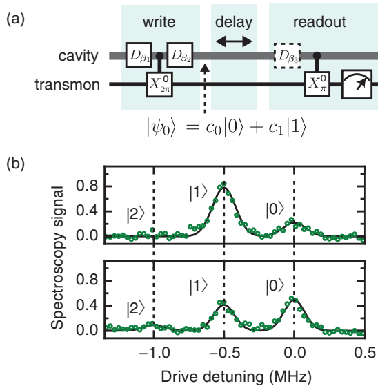
FIG. 4. Preparation of quantum resonator states. (a) Arbitrary Fock state superpositions can be written to the cavity memory using a series of displacements on the cavity and number-selective phase gates on the transmon. (b) To verify the input states for the resonator's T_1 , T_2 experiments, we perform spectroscopy on the transmon after preparing the resonator in an input state. (top) When the cavity is mostly in the first Fock state, |1\rangle , the transmon's frequency distribution reflects these statistics. By the normalized area under each peak, we determine that the population of each Fock state ( P_n ) is P_0 = 0.21 \pm 0.02 , P_1 = 0.75 \pm 0.02 , P_2 = 0.04 \pm 0.02 (bottom) After preparing a superposition of |0\rangle and |1\rangle , we find the distribution to be P_0 = 0.49 \pm 0.02 , P_1 = 0.41 \pm 0.02 , P_2 = 0.10 \pm 0.02 . This experiment alone is not sufficient to distinguish between a statistical mixture of these states and a coherent superposition. However, the phase coherence is revealed in the sinusoidal oscillations of the subsequent T_2 experiment.
