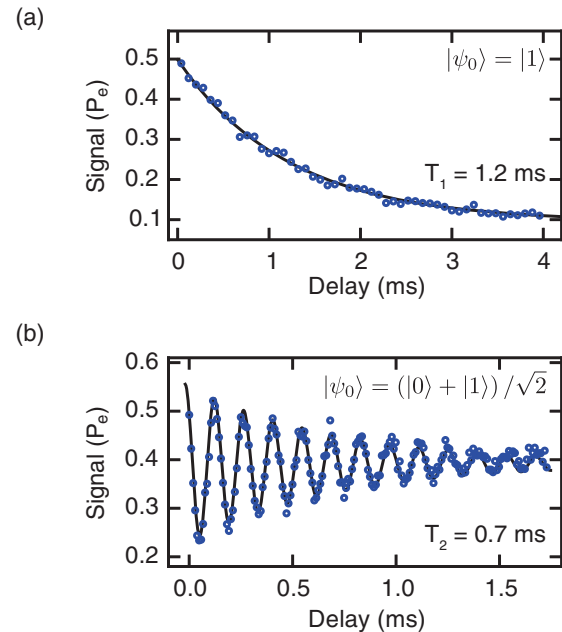
FIG. 5. Coherence of the quantum memory. (a) To prepare the Fock state |1\rangle , the optimal choice of displacements is \beta_1 = 1.14 and \beta_2 = -0.58 [37]. A single-photon decay lifetime of T_1 = 1.22 \pm 0.06 ms is extracted from the decay of the state. (b) A superposition of the Fock states |0\rangle and |1\rangle is created with \beta_1 = 0.56 and \beta_2 = -0.24 . A final displacement of \beta_1 = 0.8 \exp(j\omega t) is used to measure the coherence of the superposition. This Ramsey-like experiment yields T_2 = 0.72 \pm 0.03 ms from which we infer T_\phi \approx 1 ms.
