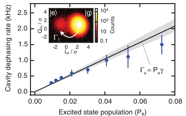
FIG. 7. Transmon-induced dephasing. (inset) A histogram of single-shot measurements of the transmon state, taken in equilibrium with a parametric amplifier, reveals a finite population in the transmon |e\rangle state of P_e = 0.8\% . In the histogram, the measurement records, \{I_m, Q_m\} , from the heterodyne detection have been scaled by the vacuum fluctuation amplitude \sigma . Quantum jumps due to this thermal bath, \Gamma_\uparrow , will dephase the state in the cavity memory at rate P_e\kappa_t . (main) The dephasing rate of the cavity memory \Gamma_\phi is measured while the transmon is excited weakly via a resonant drive. The observed total cavity dephasing rate, as a function of P_e , is in agreement with a model that assumes no intrinsic dephasing in the cavity. Error bounds have been determined using bootstrapping.
