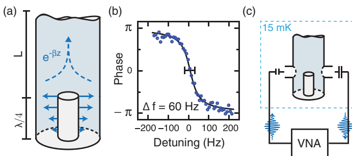
FIG. 1. High- Q coaxial microwave cavity. (a) A quarter-wave resonator is defined by short circuiting the inner and outer conductors of the coaxial transmission line at one location (bottom) and open circuiting the line a distance \lambda/4 away (upward). Fields are suppressed exponentially in the upward direction, eliminating losses at the seam. (b) The measured linear response in transmission at single-photon excitation levels show typical quality factors of Q \sim 7 \times 10^7 , corresponding to a linewidth of about 60 Hz. (c) Samples are characterized at 15 mK with a vector network analyzer (VNA).
