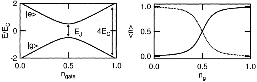
Figure 2. Energies (left) of ground and excited states of a Cooper-pair box with E_C = E_J vs. dimensionless gate charge, n_g = C_g V_g / 2e . The expectation value of a charge measurement, \langle \hat{n} \rangle , (right) for the ground (solid line) and excited (dotted line) states vs. n_g .
